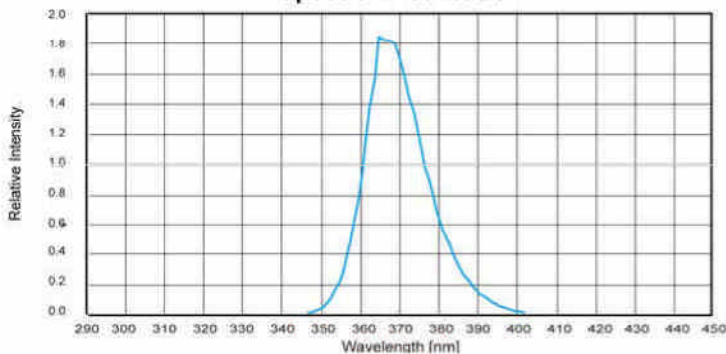
Spectral Distribution
